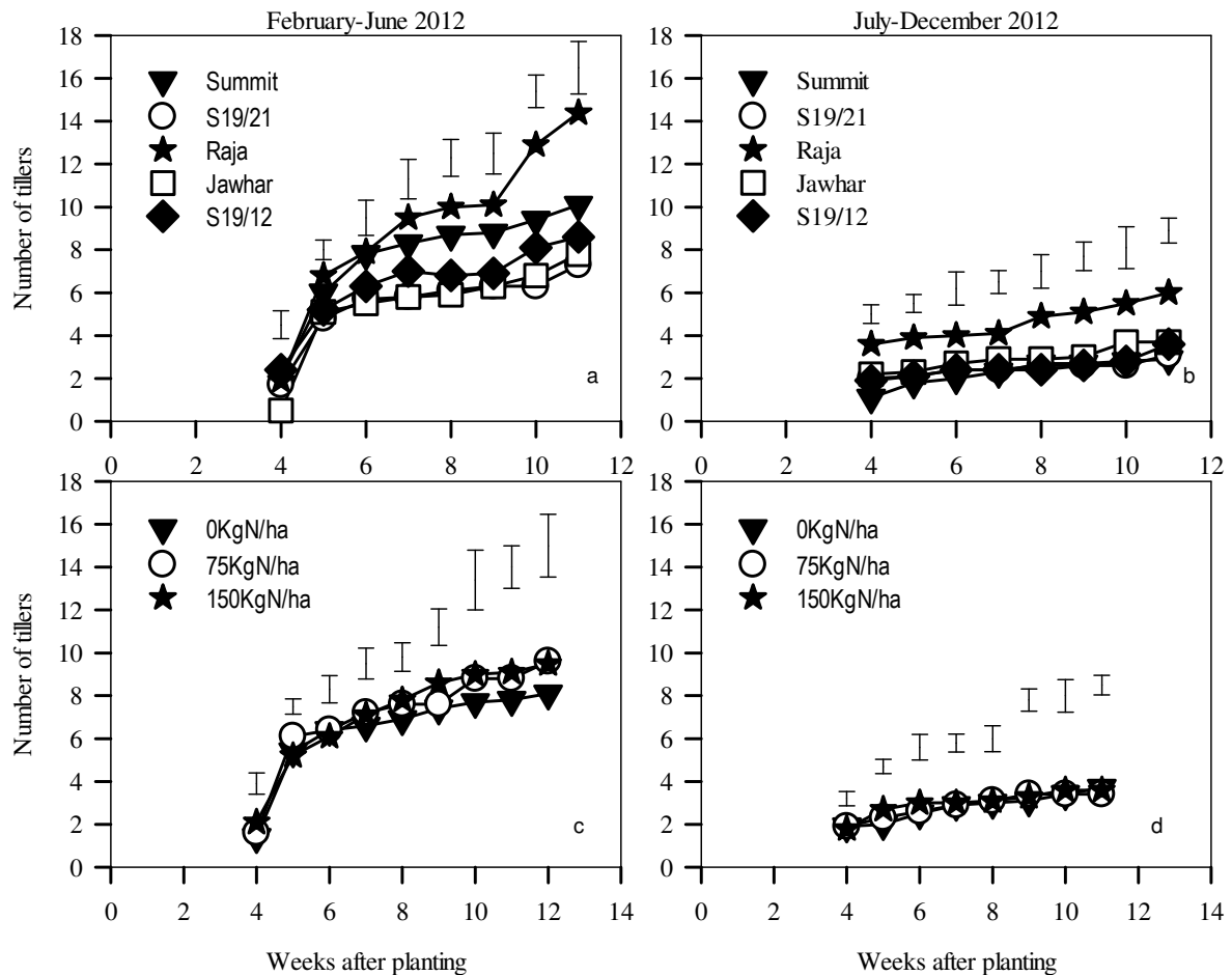
Figure 2: The number of tillers of five linseed cultivars as influenced by nitrogen fertilizer levels during February-June and July-December seasons 2012. Vertical bars show LSD 0.5 .
